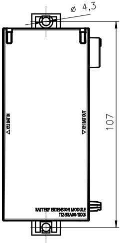
Bohrplan / Drilling plan
