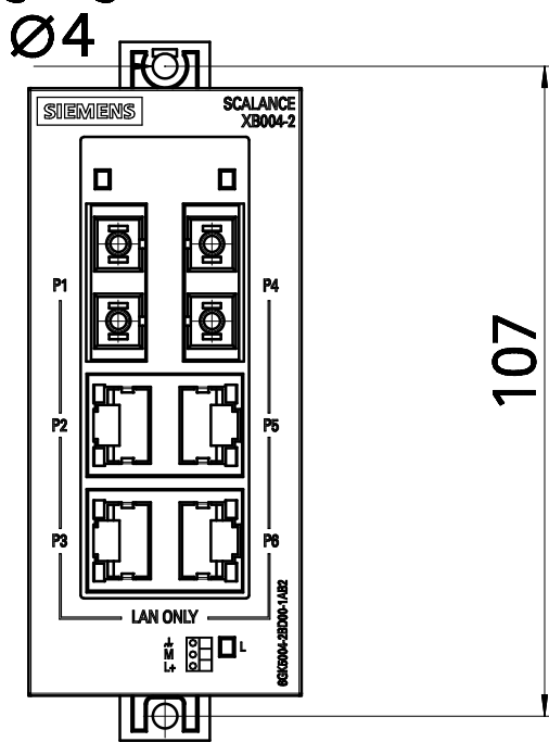
Vorne offen / Front open Alternative Befestigung / Alternative Mounting
